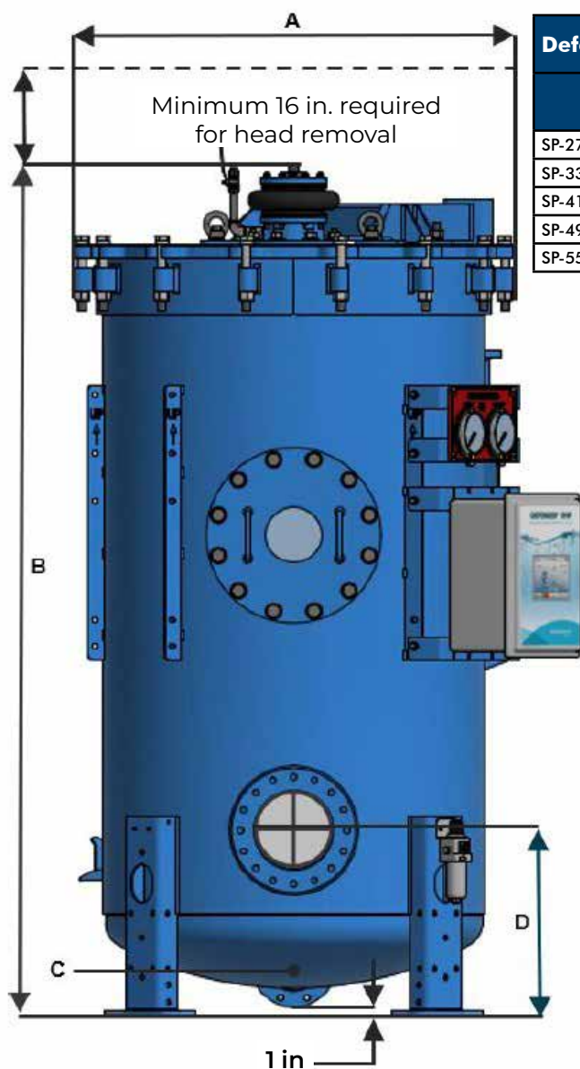
DEFENDER REGENERATIVE MEDIA FILTER - REDUCED HEIGHT
