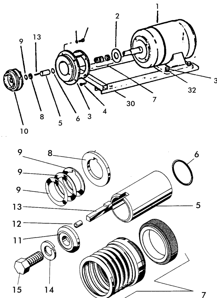
ENLARGED VIEW OF SHAFT SLEEVE AND MECHANICAL SEAL AREA.
