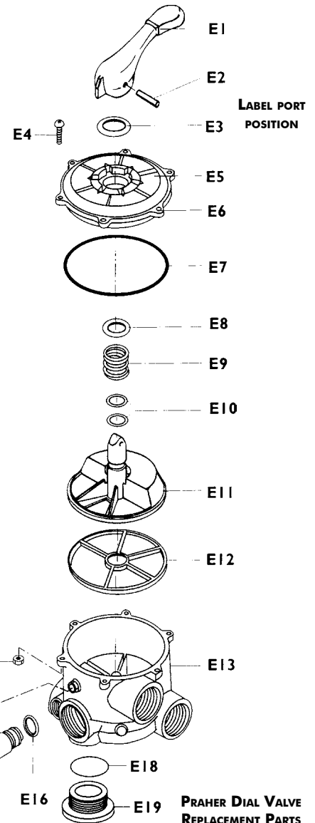
PRAHER ALL OPEN DIAL VALVE
