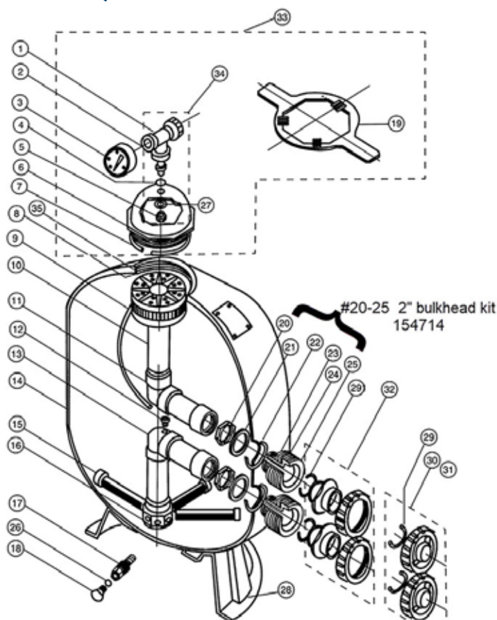
TRITON II PARTS DIAGRAM
