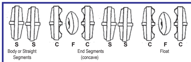
Competitor Lane Line Assembly Pattern
