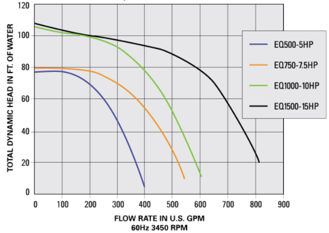
Performance curves EQ Series Pump
